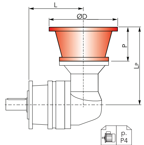
CHPL 1000 CPC - Male input shafts
