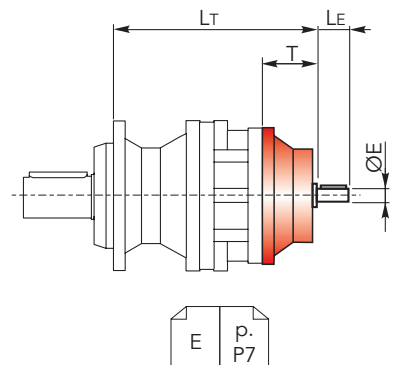
CHPL 7000 CPC - Male input shafts
