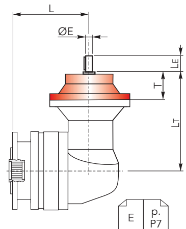
CHPL 1600 CF - Male input shafts
