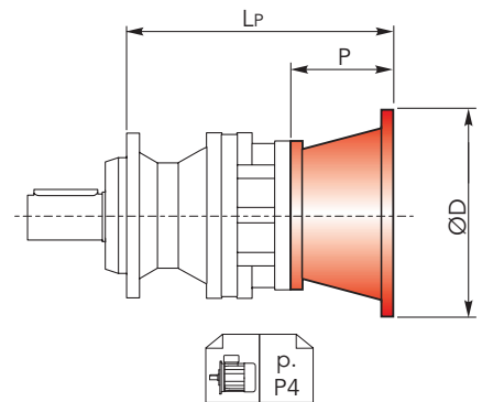
CHPL 7000 CPC- IEC Motor flanges
